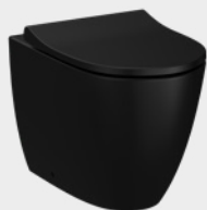
Sento back-to-wall WC pan, Rim-ex, 54cm Matt Black £470 – 7985B083-0075 H: 400mm W: 365mm P: 540mm
