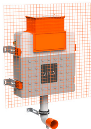
Reduced-height concealed cistern for back-to-wall WCs, 98cm, 3/6 litre
